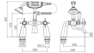
Bath Shower Mixer NV126
