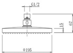
Islington 200mm Shower Head NV170
