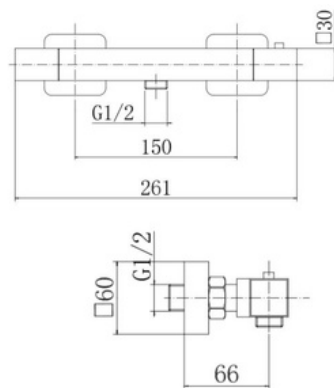
Mayfair Square Bar Valve NV166 Flow Rates: 0.5 Bar 4.5 | 1 Bar 6.2 | 5 Bar 12.1
