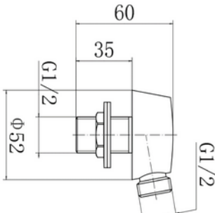
Round Outlet Elbow NV200 NV200-MB NV200-BB
