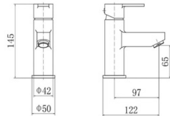
Basin Mixer NV002 NV002-MB
